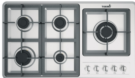
TS 502 Size 86 x 50 cm Gas burner 5 Finishing Satin Top panel 304SS
