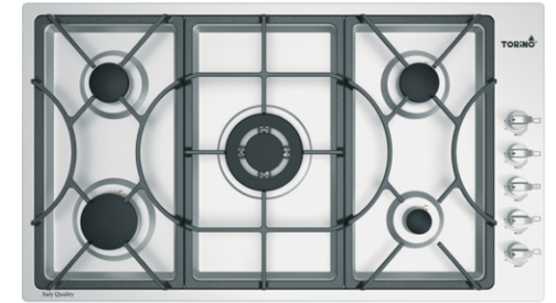
TS 515 Size 89 x 51 cm Gas burner 5 Finishing Satin Top panel 304SS
