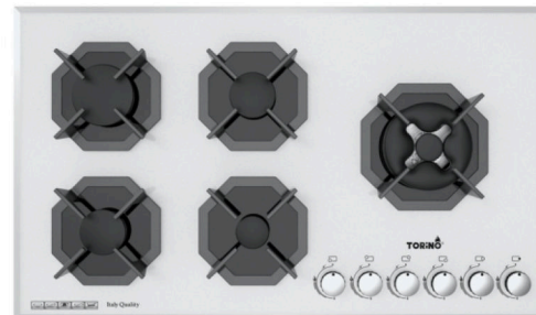
TG 528W Size 88 x 52 cm Gas burner 5 Color Tempered White glass Burner Dual Triple ring burner Safety valve 6PCS
