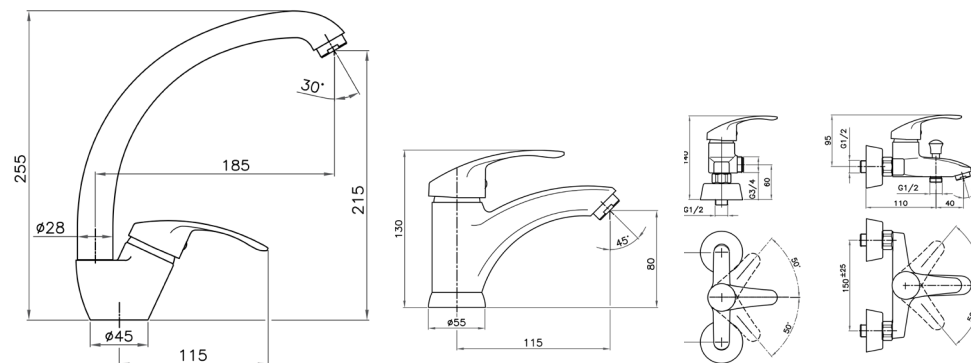
▲ Bathroom Faucet
