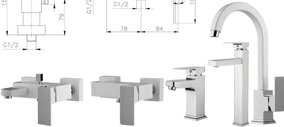
▲ Bathroom Faucet
